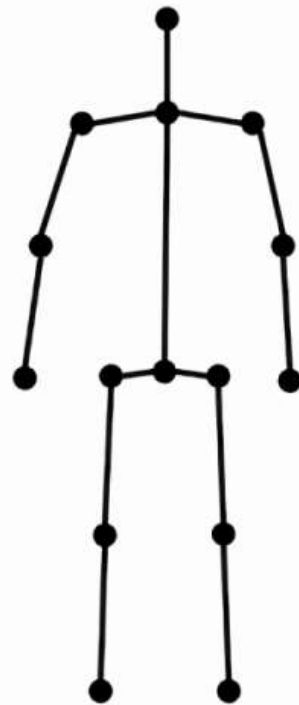
skeleton-based model
