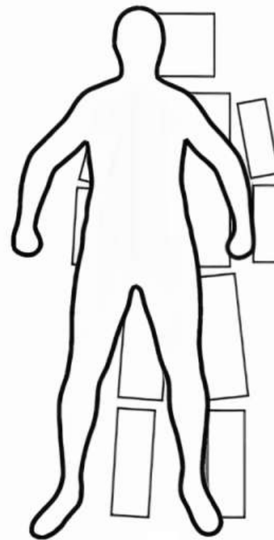
contour-based model
