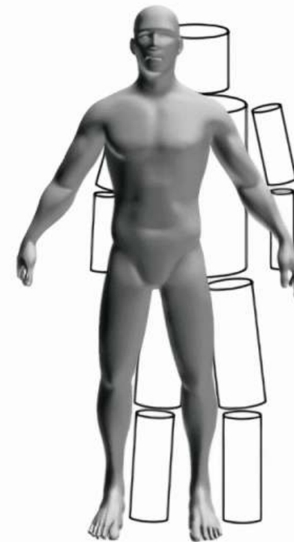
volume-based model
